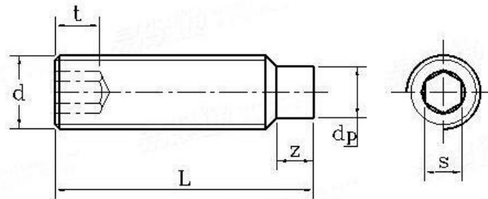
DIN915 Hexagon socket set screws with dog point
